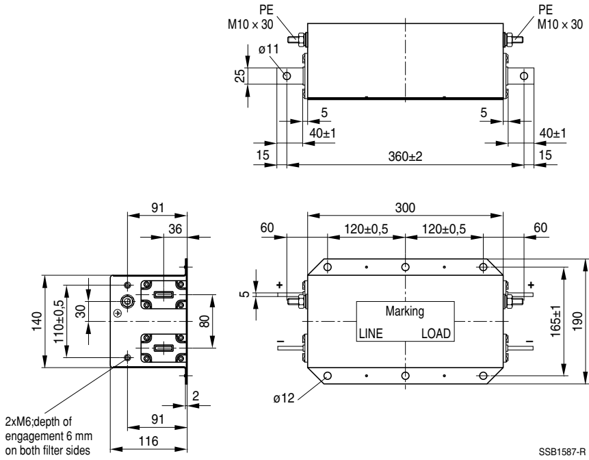
Dimensional drawing B84142-A250-S**
