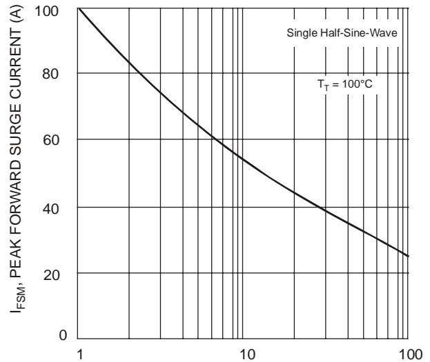
Single Half-Sine-Wave T_T = 100^\circ\text{C} Fig. 4 Max Non-Repetitive Peak Forward Surge Current
