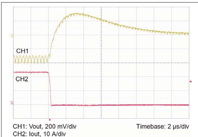
Figure 11 — 25-0 A load step with 47 \mu F input capacitance.
