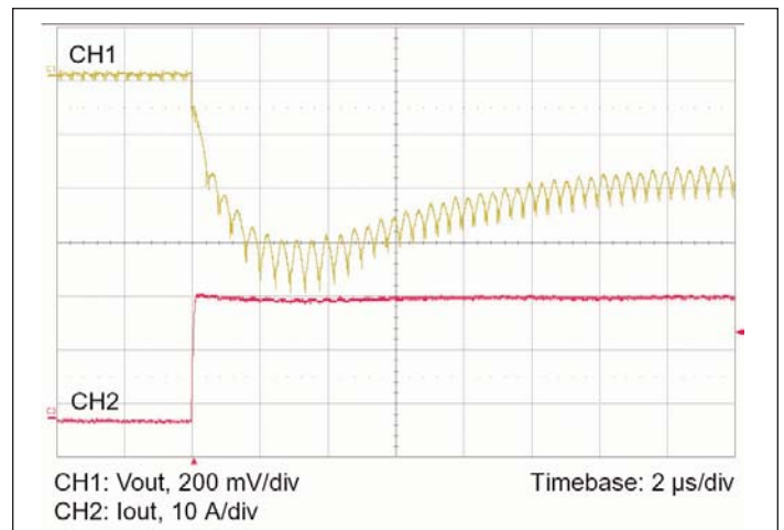
Figure 10 — 0-25 A load step with 47 \mu F input capacitor and no output capacitor.
