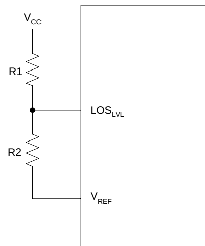
LOS_{LVL} CIRCUIT
