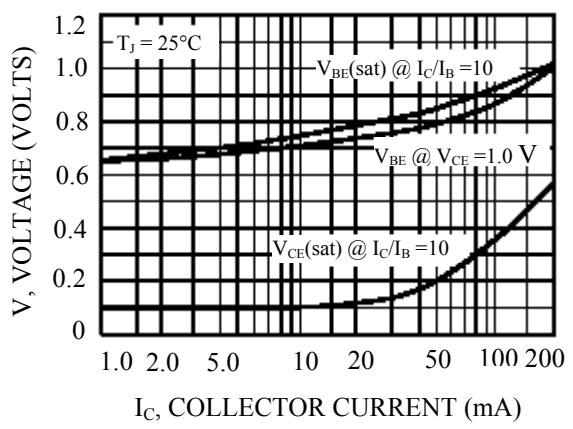
Figure 3. "ON" Voltages
