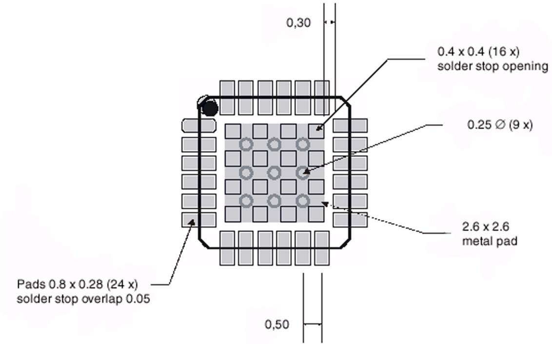
Figure 11-1. Recommended Footprint (QFN24 - 4 mm × 4 mm)
