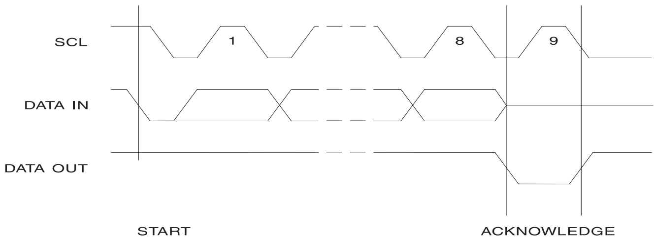
Figure 6. Output Acknowledge
