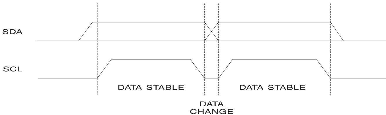
Figure 4. Data Validity
