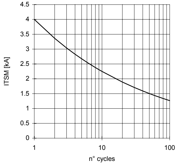
SURGE CHARACTERISTIC T_j = 150\text{ }^\circ\text{C}
