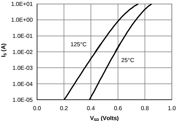
Figure 6: Body-Diode Characteristics
