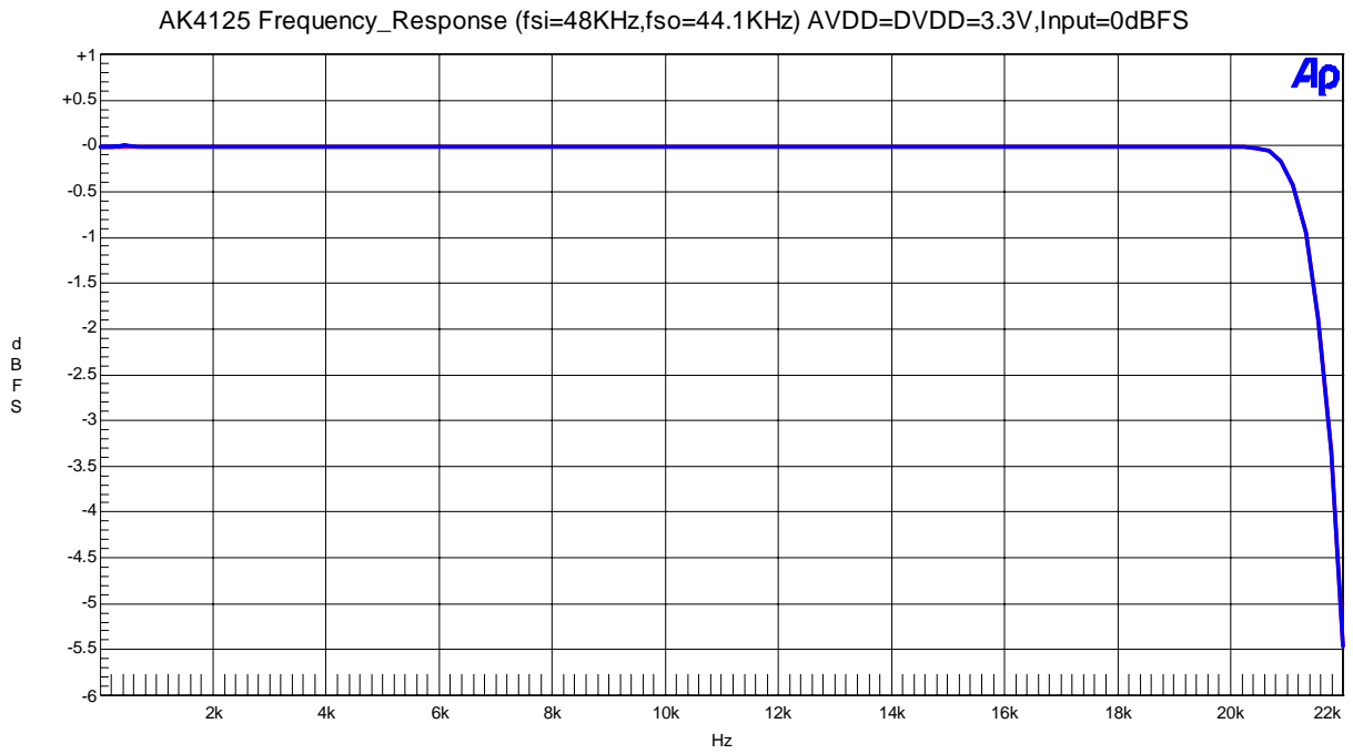
Fig 5. Frequency Response
