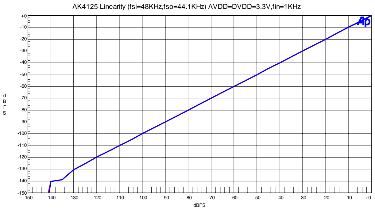
Fig 4. Linearity
