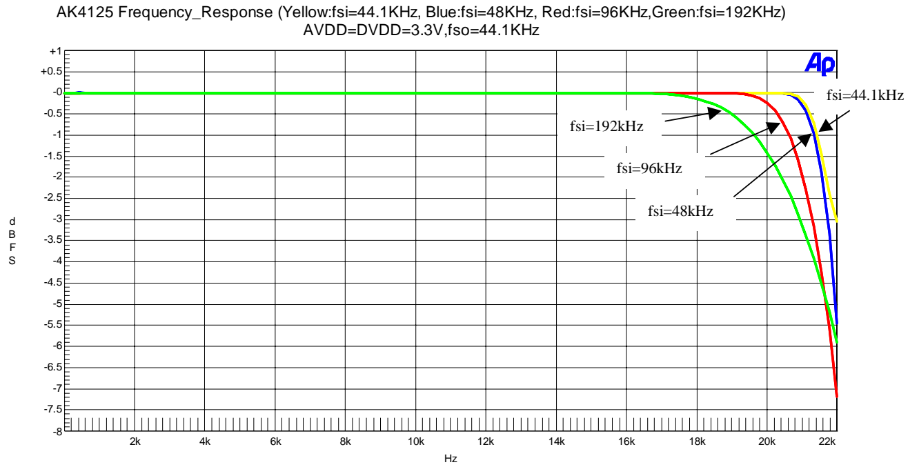
Fig 9. Frequency Response
