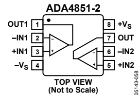
Figure 2. ADA4851-2, 8-Lead MSOP (RM-8)
