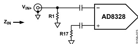
Figure 23. Single-Ended Circuit
