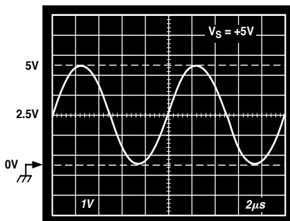
Figure 1. Output Swing: Gain = -1 , R_L = 2 k\Omega
