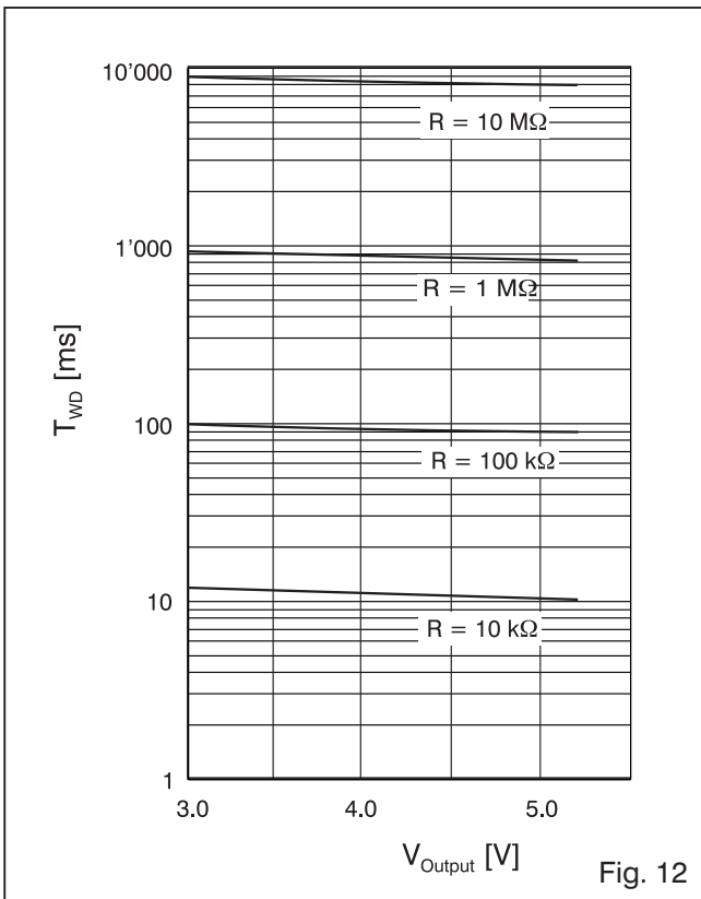
T_{WD} versus V_{OUTPUT} at T_J = +25^\circ C
