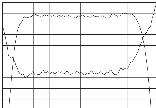
Horizontal: 1.5 MHz/Div Vertical: 1 dB/Div Vertical: 5 deg/Div
