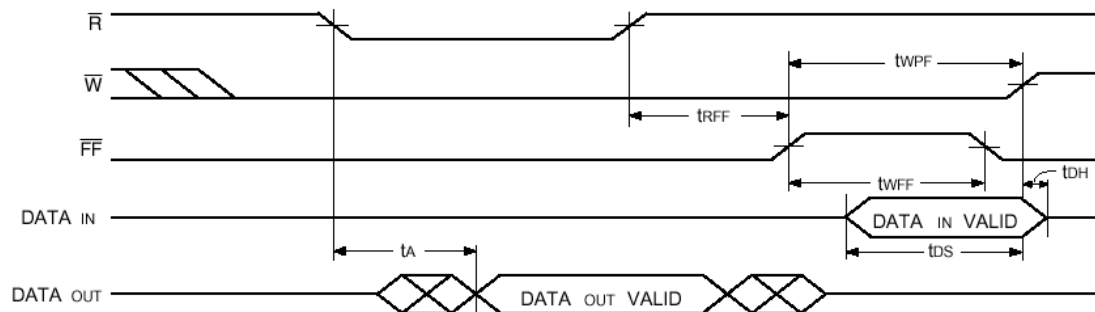
FIGURE 12. WRITE DATA FLOW FOR THROUGH MODE
