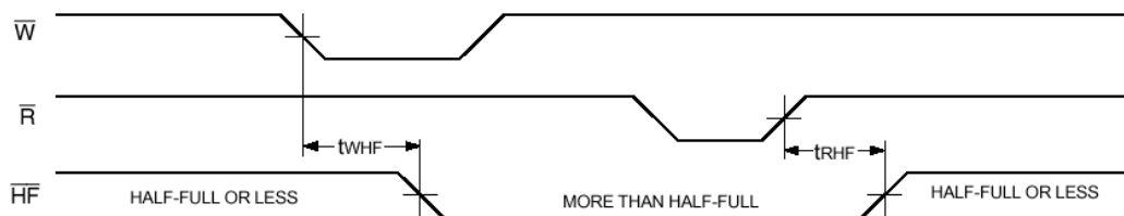
FIGURE 9. EXPANSION OUT
