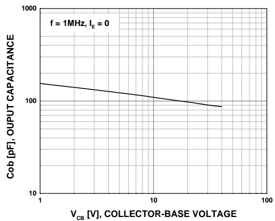
Figure 6. Output Capacitance
