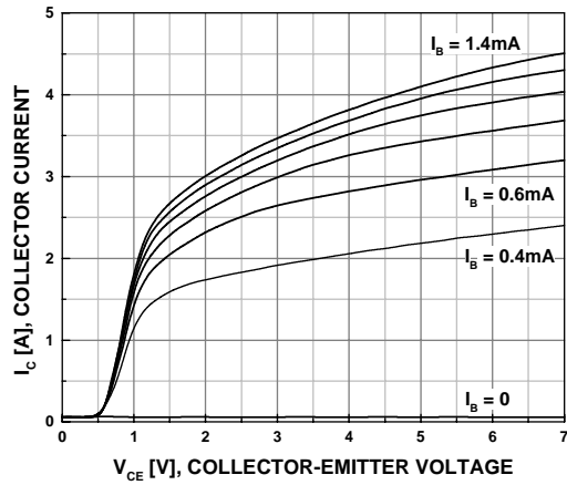
Figure 1. Static Characteristic
