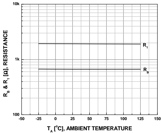
Figure 5. R_B , & R_1 vs. Ambient Temperature
