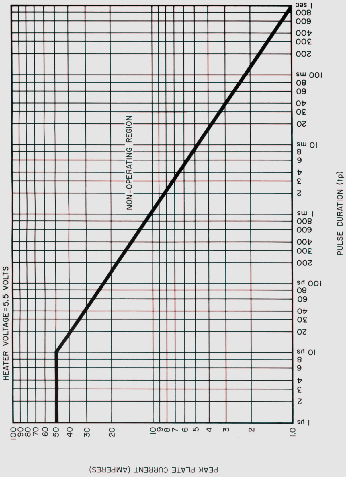
PULSE DERATING DATA, TYPE 3CPX1500A7 - PULSE MODULATOR OR REGULATOR SERVICE
