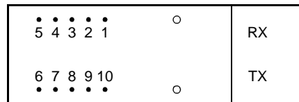
Figure 1. 2417J4A Transceiver, 10-Pin Configuration, Top View
