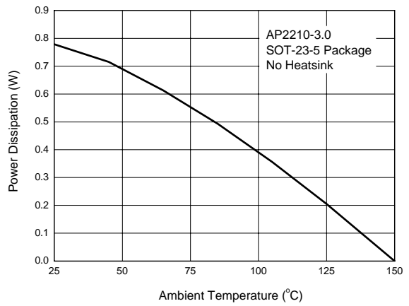
Figure 17. Power Dissipation vs. Ambient Temperature
