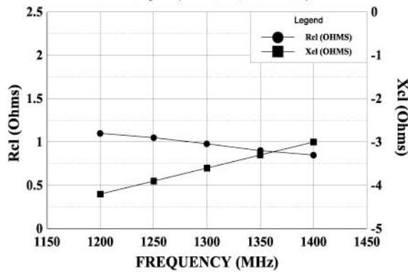
LOAD IMPEDANCE vs FREQUENCY
