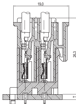
TERMINAL ASSEMBLY DRAWING
