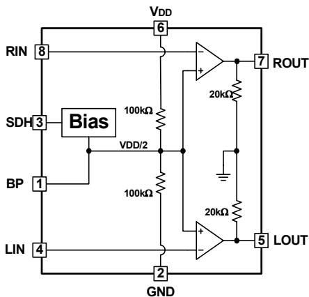
FAN7005MU(8MSOP)
