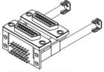
DUAL BOARDLOCKS
