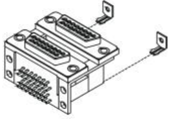
SINGLE BOARDLOCK
