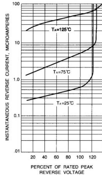
FIG. 4 - TYPICAL REVERSE CHARACTERISTICS
