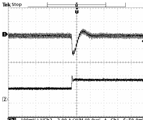
Transients 50% to 100% load 0.75 Vdc output
