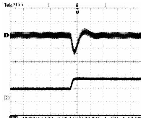
Transients 50% to 100% load 1.8 Vdc output
