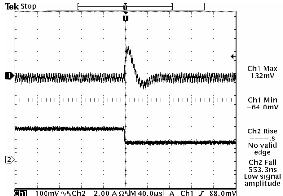
Transients 100% to 50% load 0.75 Vdc output
