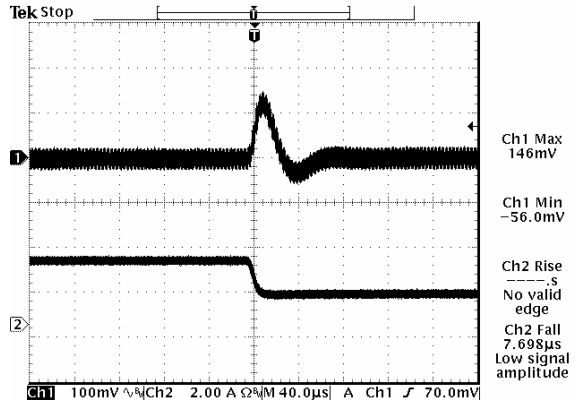
Transients 100% to 50% load 1.8 Vdc output
