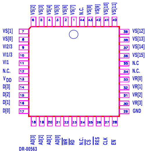
Package: PLCC-44
