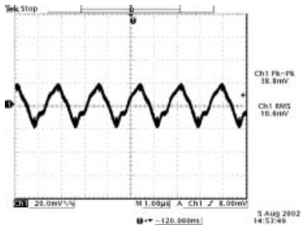
Ripple and noise at full load and 3.3Vdc input, 5Vdc output and T_a=25^\circ\text{C}
