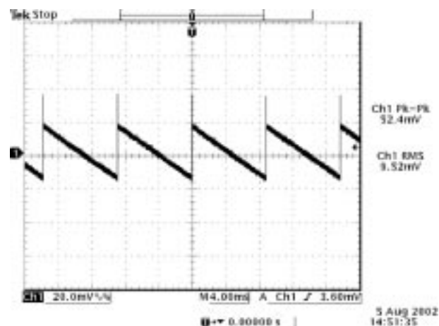
Ripple and noise at no load and 3.3Vdc input, 5Vdc output and T_a=25^\circ\text{C}
