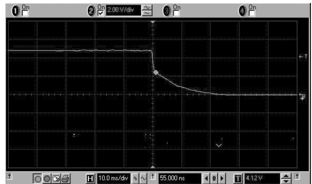
Fall Time (PWM mode): V_{in} = 3.5V ; V_{TP} = 5V ; I_{out} = 1A
