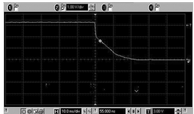
Fall Time (PWM mode): V_{in} = 3V ; V_{TP} = 3.3V ; I_{out} = 1A
