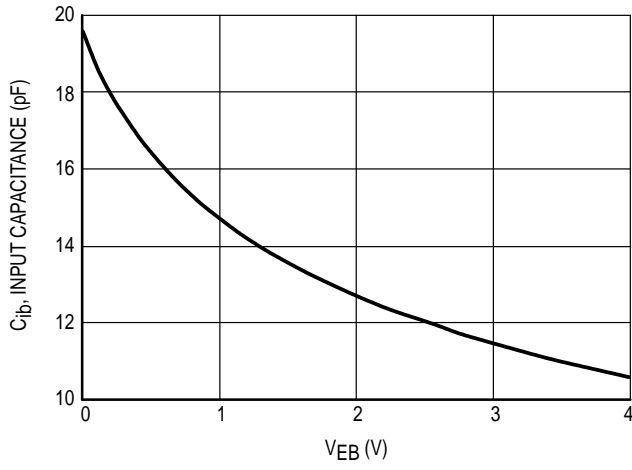
Figure 6. Capacitance
