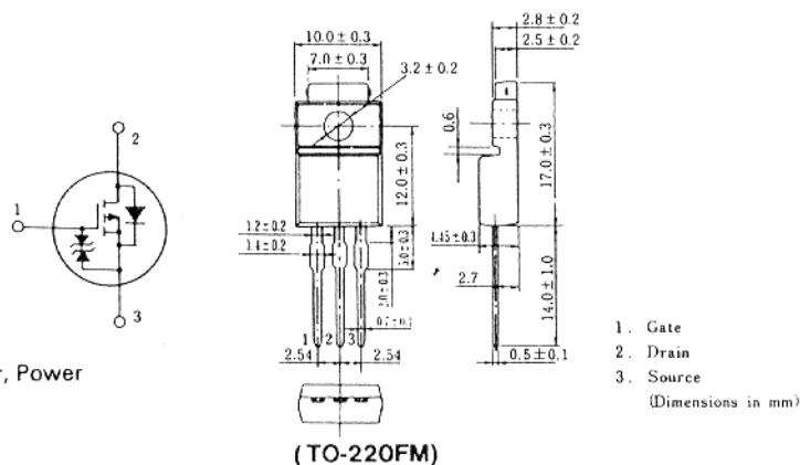
(TO-220FM)
