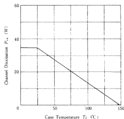
(TO-220FM)
