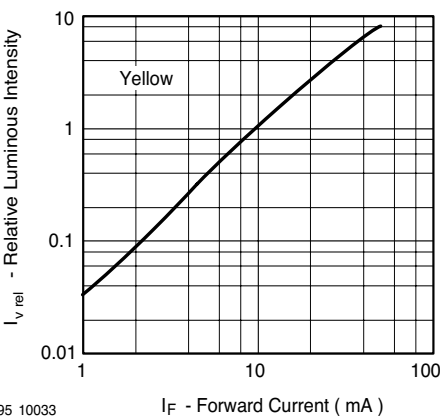
95 10033 I_F - Forward Current (mA) Figure 17. Relative Luminous Intensity vs. Forward Current
