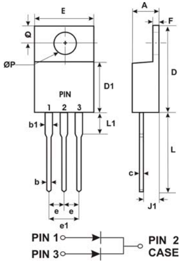
TO-220AB
