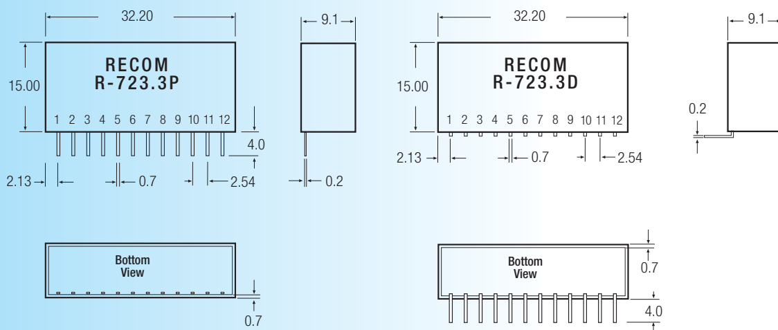
SIP12 PIN Package
