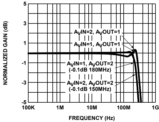
FIGURE 7. GAIN vs FREQUENCY FOR VARIOUS GAIN COMBINATIONS
