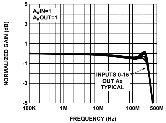
FIGURE 4. GAIN vs FREQUENCY FOR VARIOUS INVERTING INPUTS
