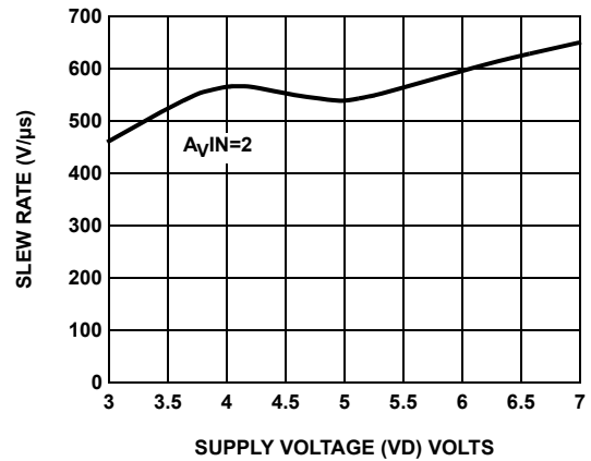
FIGURE 24. SLEW RATE vs SUPPLY (VD)
