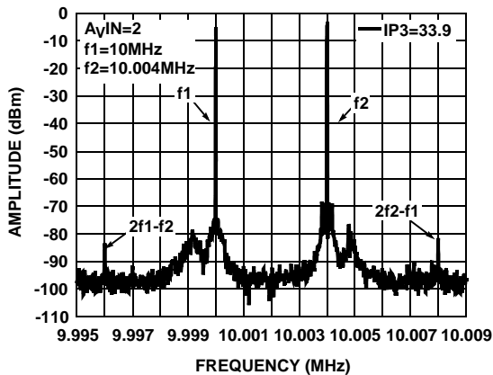
FIGURE 41. IP3 A_{vIN} = 2 BLUE CHANNEL
