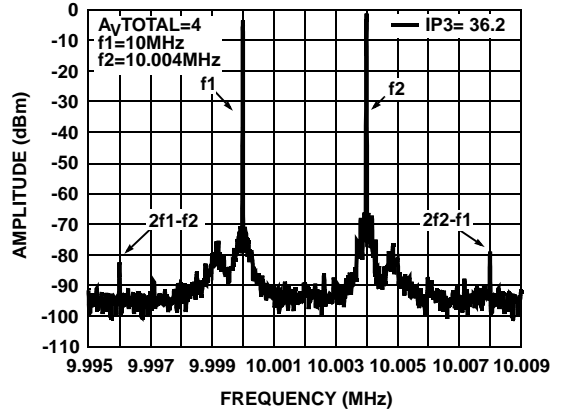
FIGURE 40. IP3 A_{vTOTAL} = 4 BLUE CHANNEL
