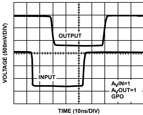
FIGURE 27. LARGE SIGNAL NEGATIVE PULSE RESPONSE
