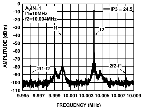
FIGURE 42. IP3 A_{vIN} = 1 BLUE CHANNEL
