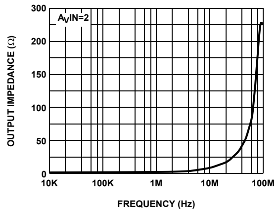
FIGURE 22. OUTPUT IMPEDANCE
