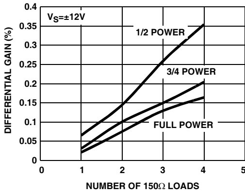
FIGURE 37. DIFFERENTIAL GAIN
