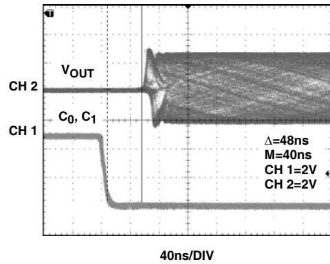
FIGURE 40. ENABLE RESPONSE
