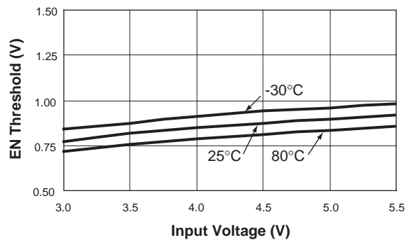
EN Threshold vs. Input Voltage
