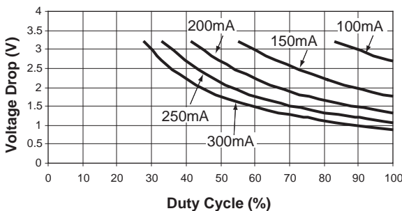
Device Duty Cycle vs. V_{DROP} ( V_{DROP} = 2.8V @ 85^{\circ}C )
