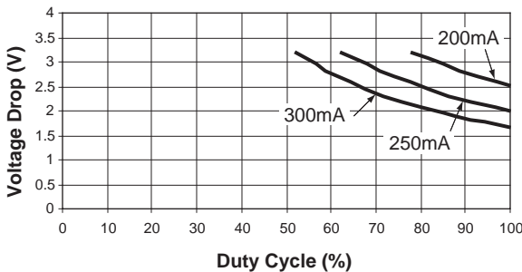
Device Duty Cycle vs. V_{DROP} ( V_{DROP} = 2.8V @ 50^{\circ}C )
