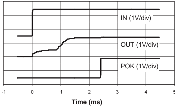
Power-Up With 1mA Load
