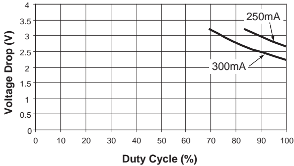
Device Duty Cycle vs. V_{DROP} ( V_{DROP} = 2.8V @ 50^{\circ}C )
