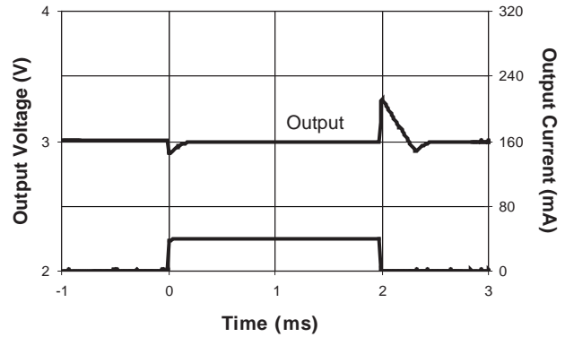
Load Transient – 1mA/40mA
