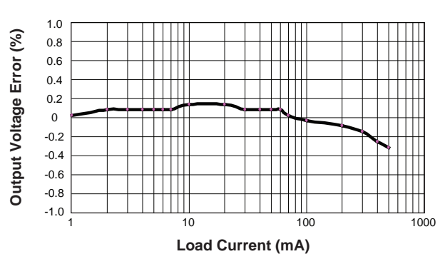
Load Regulation ( V_{IN} = 3.6V ; V_{OUT} = 1.8V ; L = 2.2\mu H )
