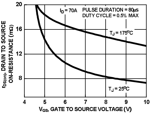
Figure 9. On-Resistance vs Gate to Source Voltage
