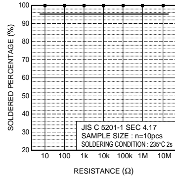
Fig.10 Solderability
