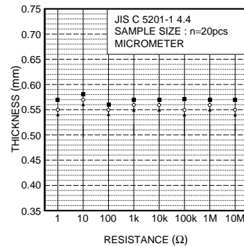
Fig.4 Dimensions (thickness)
