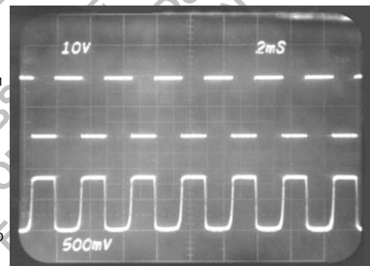
Figure 7. Output Pulse for an 8 Tooth Gear
