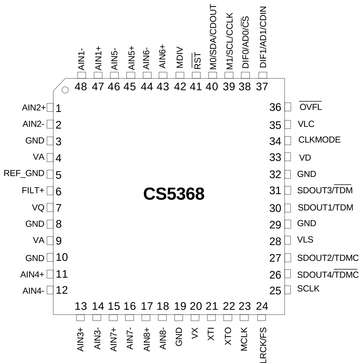
Figure 1. CS5368 Pinout
