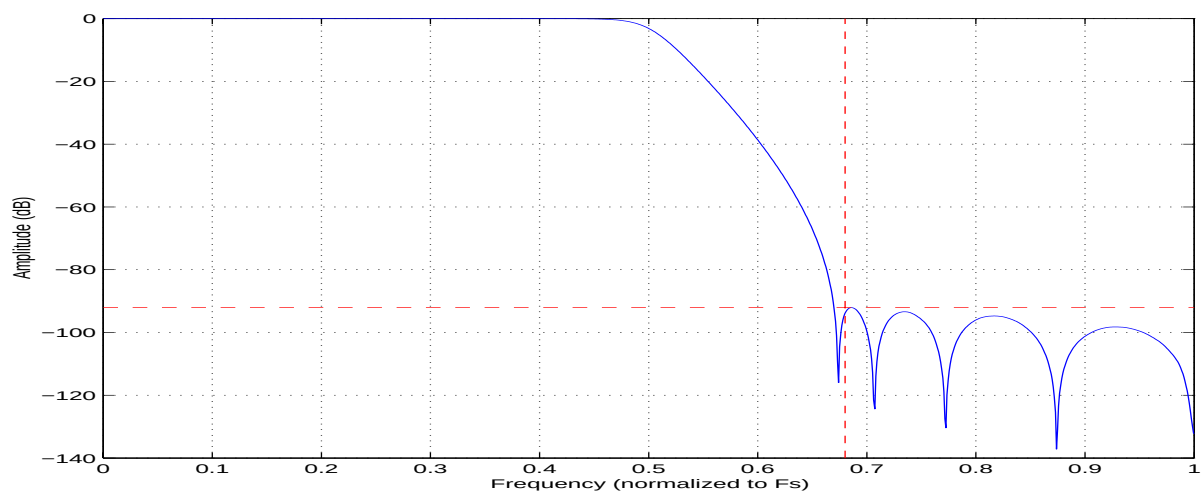
Figure 22. DSM Stopband
