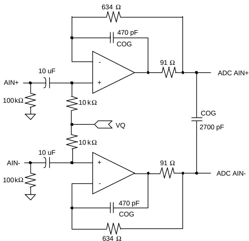
Figure 7. Recommended Analog Input Buffer
