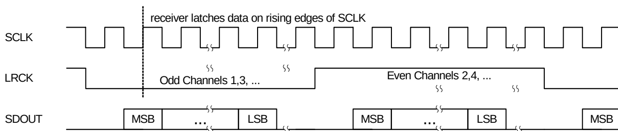
Figure 13. I²S Format
