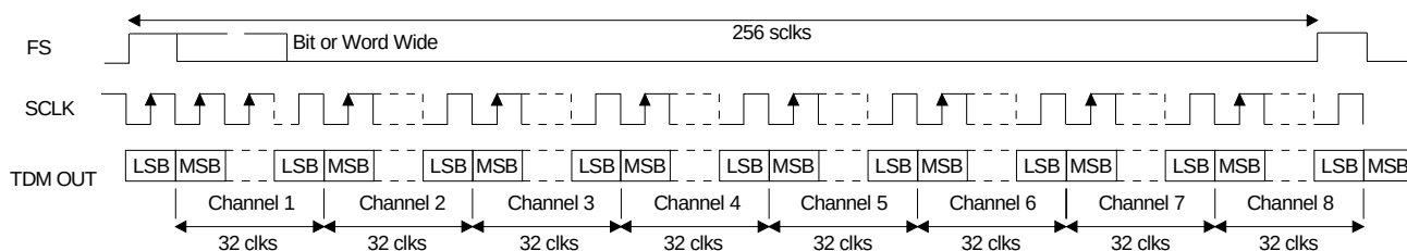
Figure 14. TDM Format
