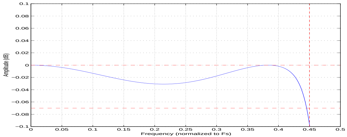
Figure 19. DSM Passband
