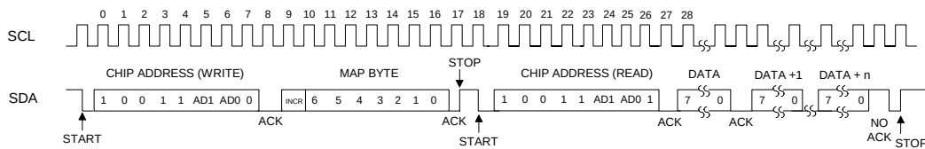
Figure 17. I²C Read Format
