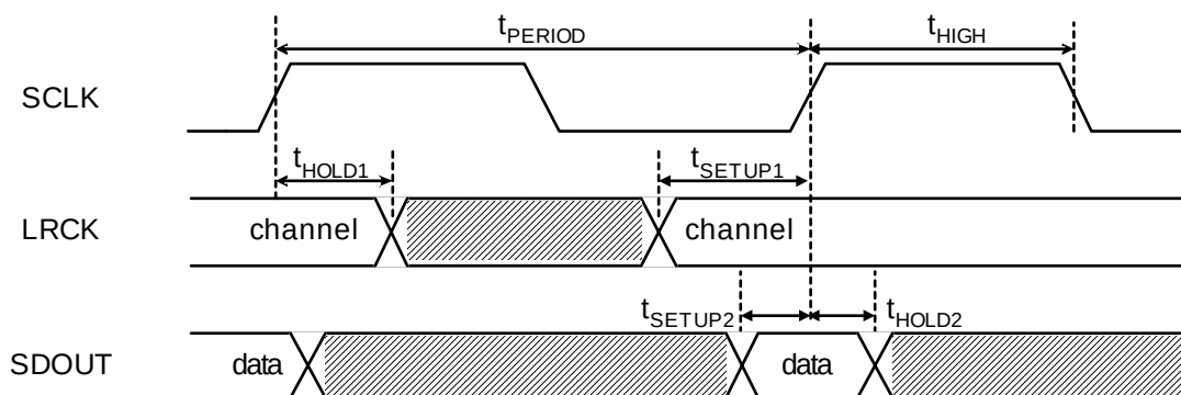
Figure 2. I 2 S/LJ Timing
