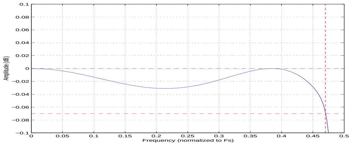
Figure 18. SSM Passband
