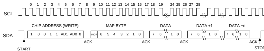
Figure 16. I²C Write Format
