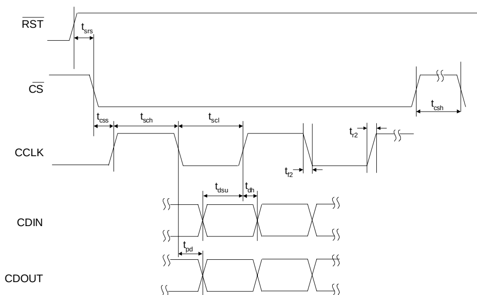
Figure 5. SPI Timing
