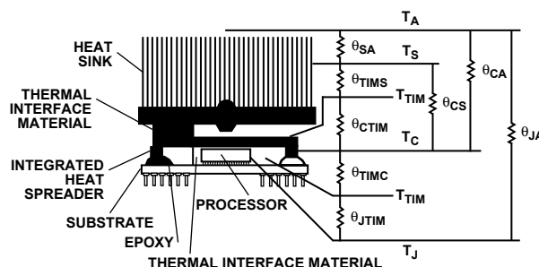
Figure 62. Thermal Model
