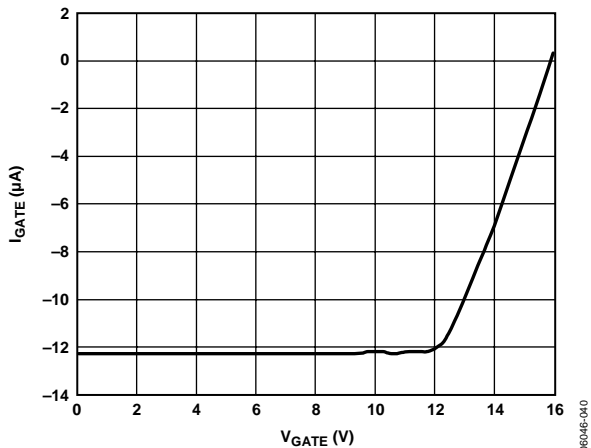
Figure 11. Gate Pull-Up Current vs. Gate Voltage at V_{CC} = 5\text{ V}
