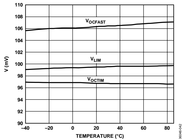
Figure 23. V OCTIM , V LIM , V OCFAST vs. Temperature
