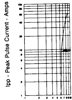
FIGURE 4 TYPICAL CLAMPING VOLTAGE ( V_C ) VS. PEAK PULSE CURRENT ( I_{PP} )
