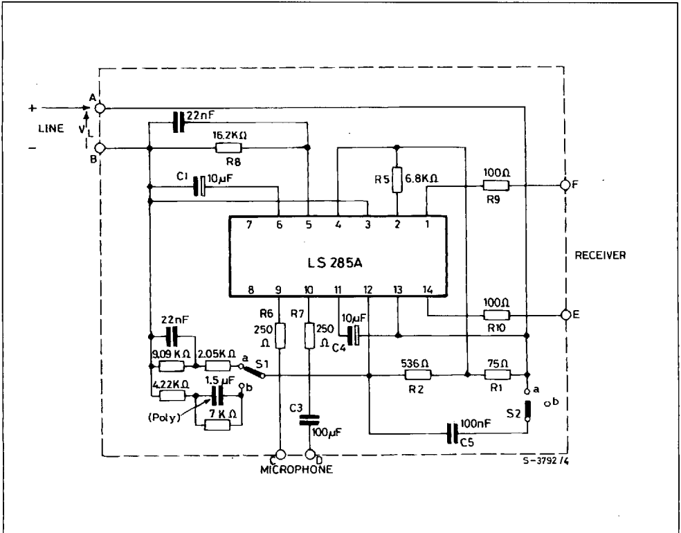
Figure 1 : Test Circuit.
