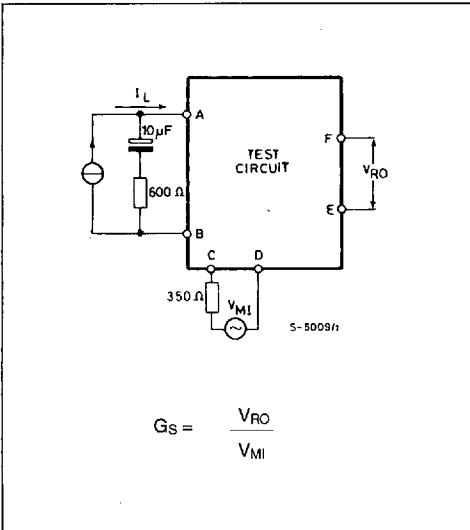
Figure 4 : Sidetone.
