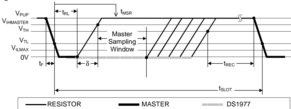
Figure 10. Read-data Time Slot
