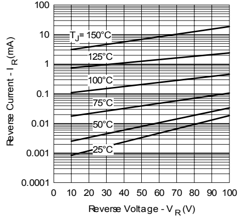
Fig. 2 - Typical Values of Voltage Current Vs. Reverse Voltage
