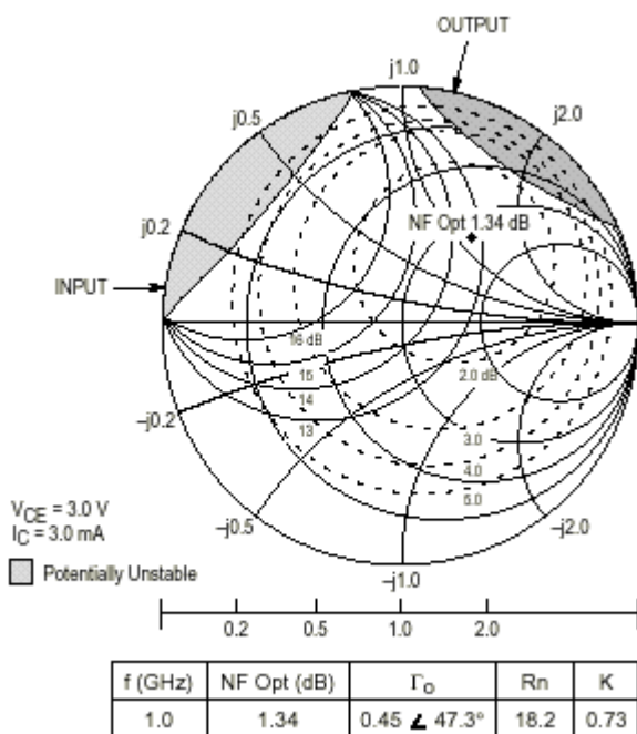
Fig. 21 Constant Gain & Noise Figure Coutours
